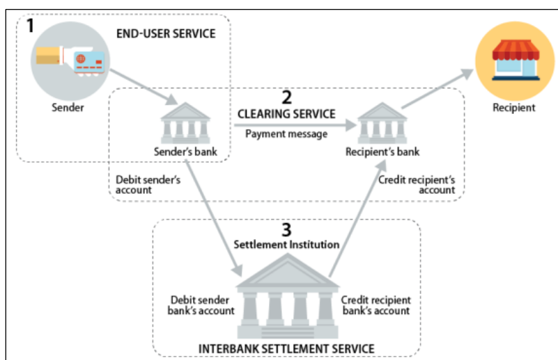
Figure 1. Traditional Payments
